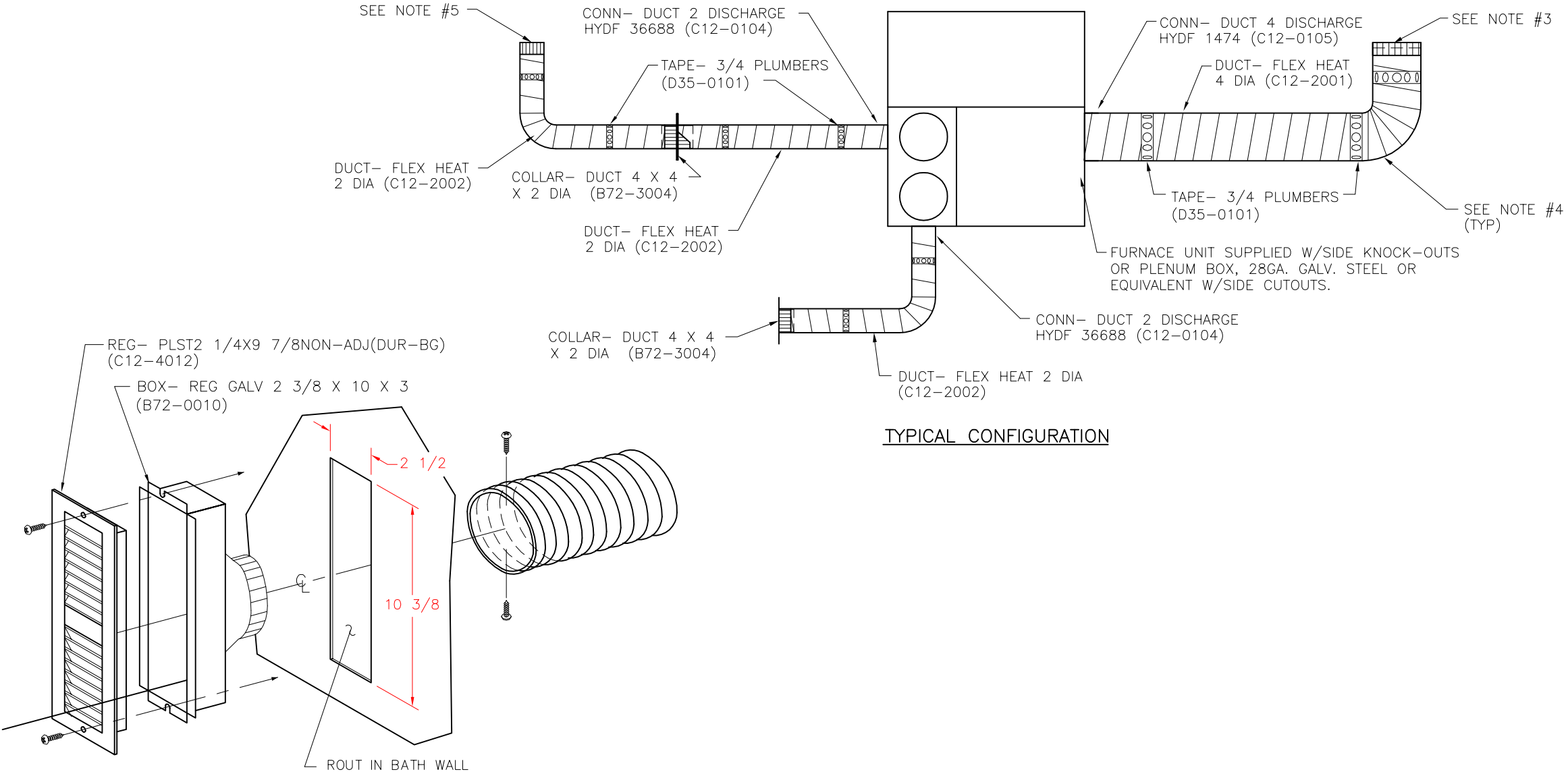
REGISTER DETAIL SCALE: 2 1/2" = 1'-0"
