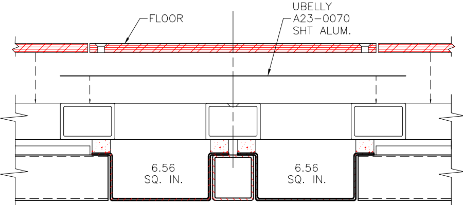
ALTERNATIVE CROSSOVER DETAIL
