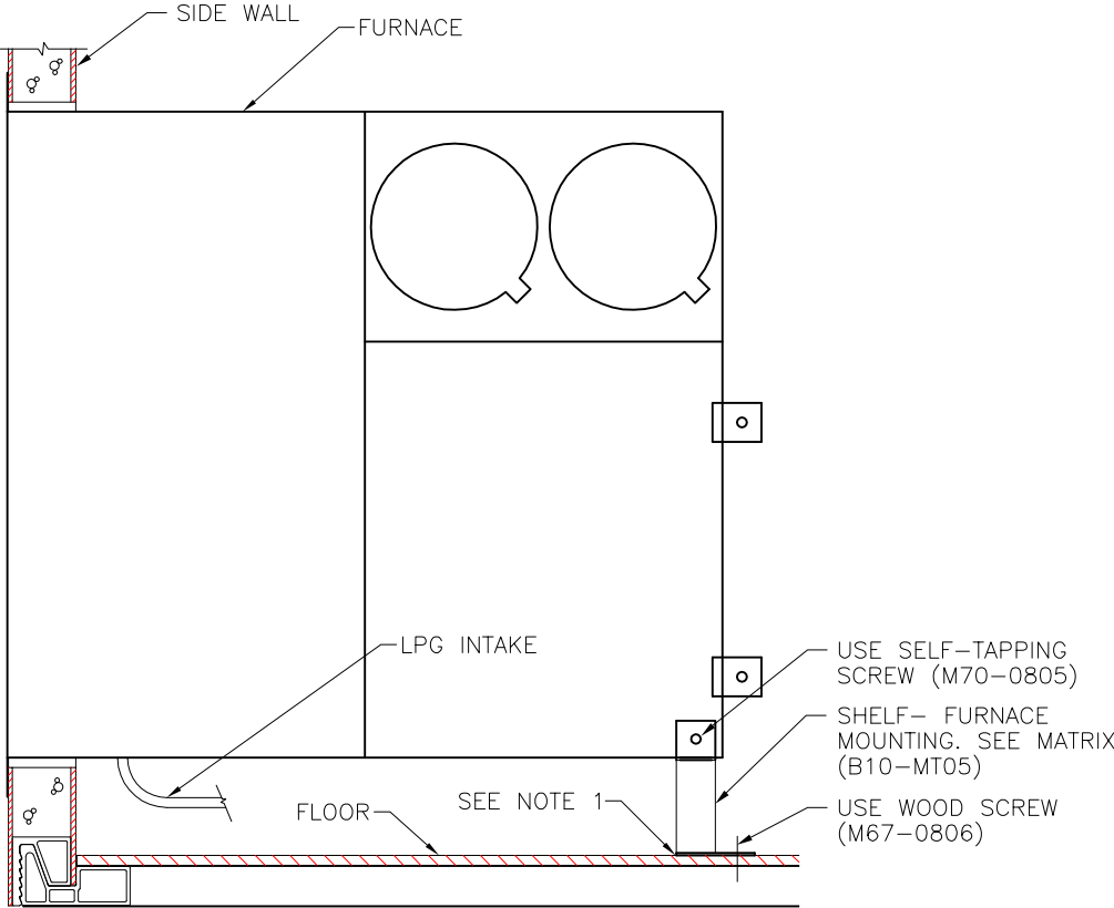
VERTICAL MOUNTING OF FURNACE (SIDE VIEW)
